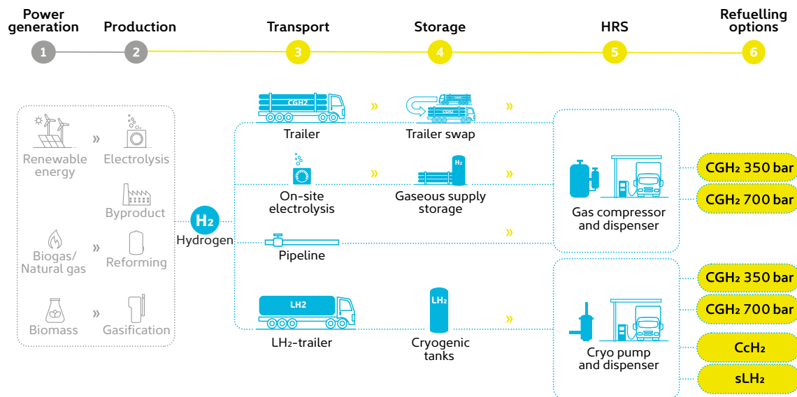
Figure 6 – The hydrogen supply chain
